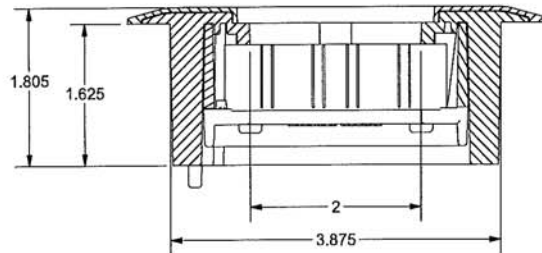
SECTION A-A SCALE 3/4
