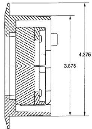
SECTION B-B SCALE 3/4
