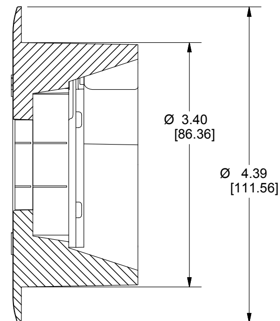
SECTION A-A SCALE 3/4
